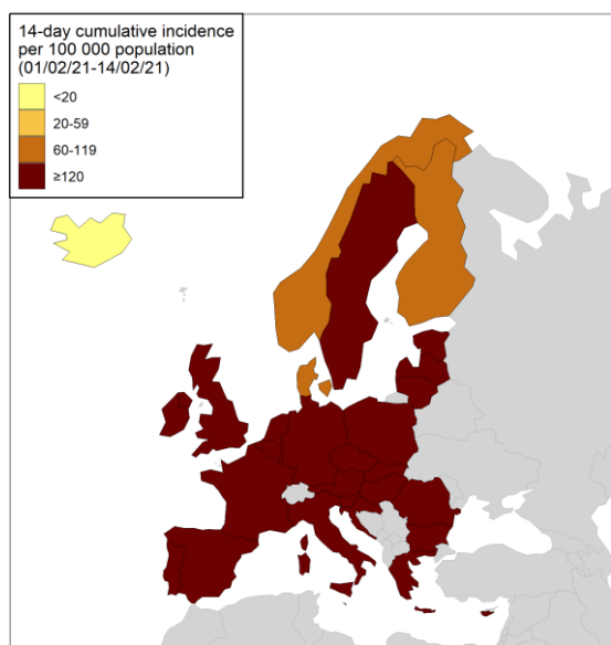
Distribution of cumulative confirmed cases per 100 000 inhabitants (01/02/21 - 14/02/21)
