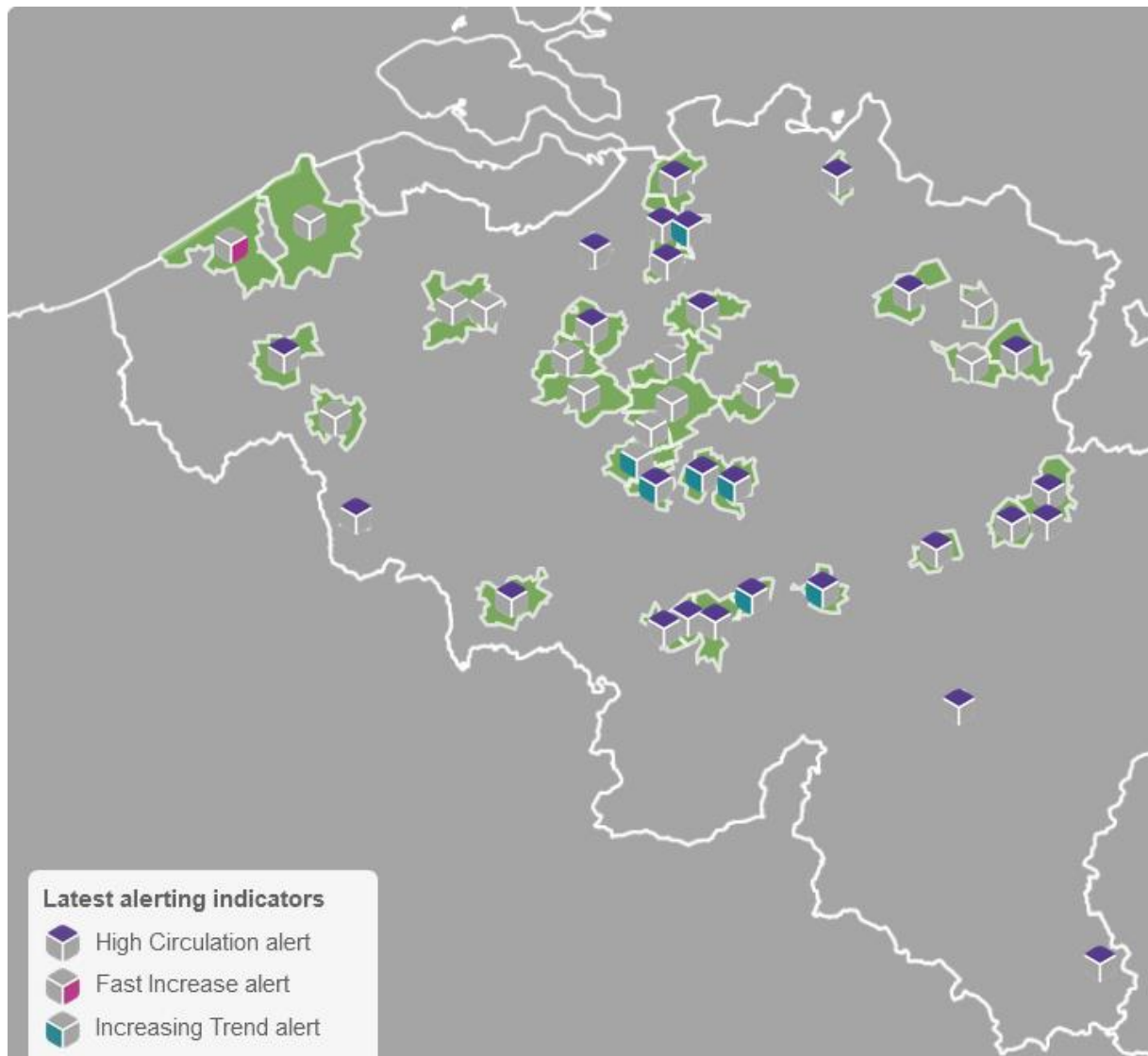
Figure 2: The geographical location of the covered areas with the corresponding status of the three alerting indicators: High circulation, Fast Increase and Increasing trend. If an indicator is in alert its corresponding slice is displayed in its colour (see legend) whereas when not in alert the same slice is greyed out. When no data is available for an area, the 3 slices are displayed in white. The names of the covered areas with respect of their localization can be found in Figure 1.
