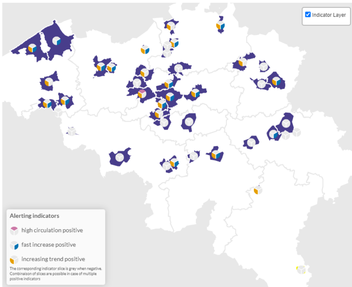
Figure 4: Localization of the covered areas (violet polygons) by the wastewater surveillance in Belgium. In each area, the fulfillment of the High circulation, Fast increase and Increasing trend indicator is indicated by a pink, blue and yellow slice, respectively. The names of the covered areas with respect of their localization can be found in Figure 1.
